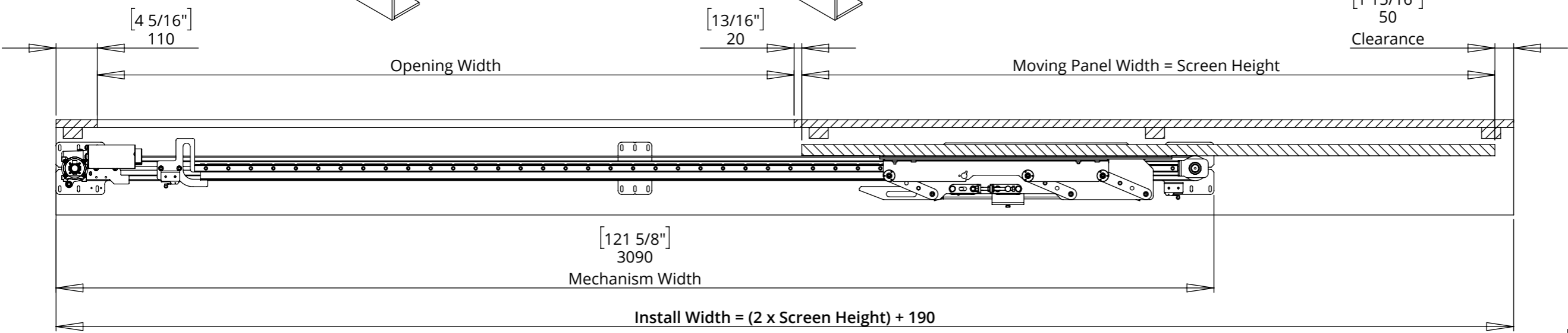
SECTION B-B Maximum Screen Height
