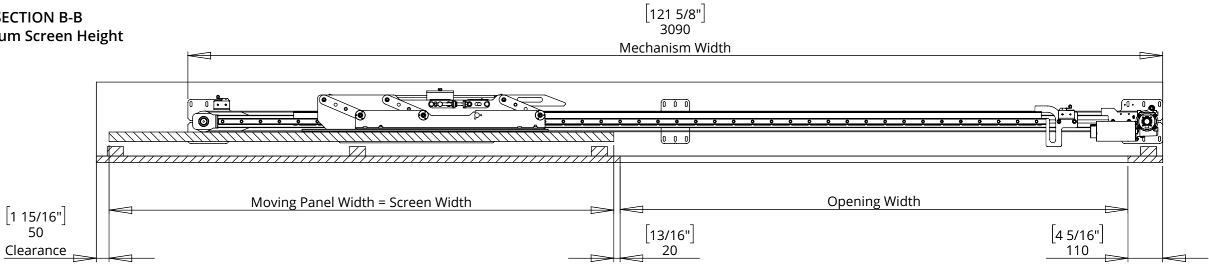
SECTION B-B Maximum Screen Height
